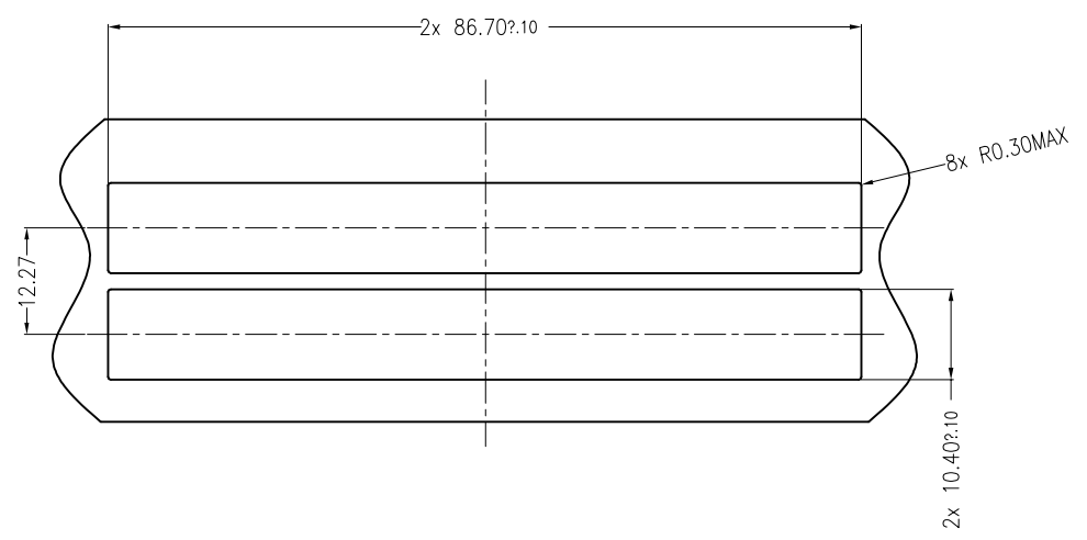
RECOMMENDED BEZEL CUT-OUT BELLY TO BELLY APPLICATIONS
